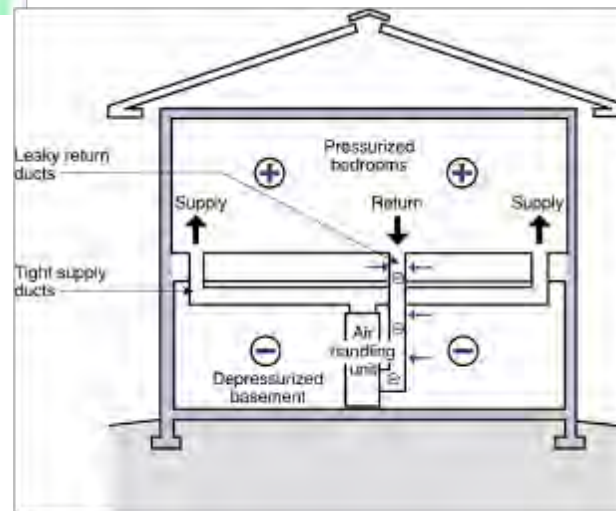
Mechanical Systems
