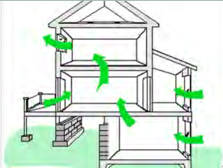
Stack Effect
