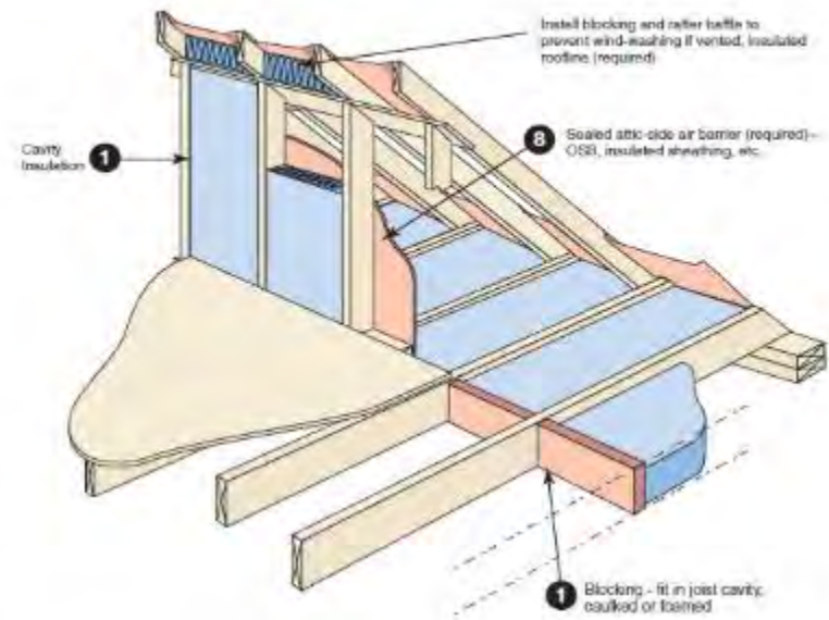
Attic knee-walls
