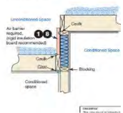
Two-level attic
